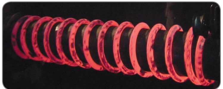
Hot wound coiling
